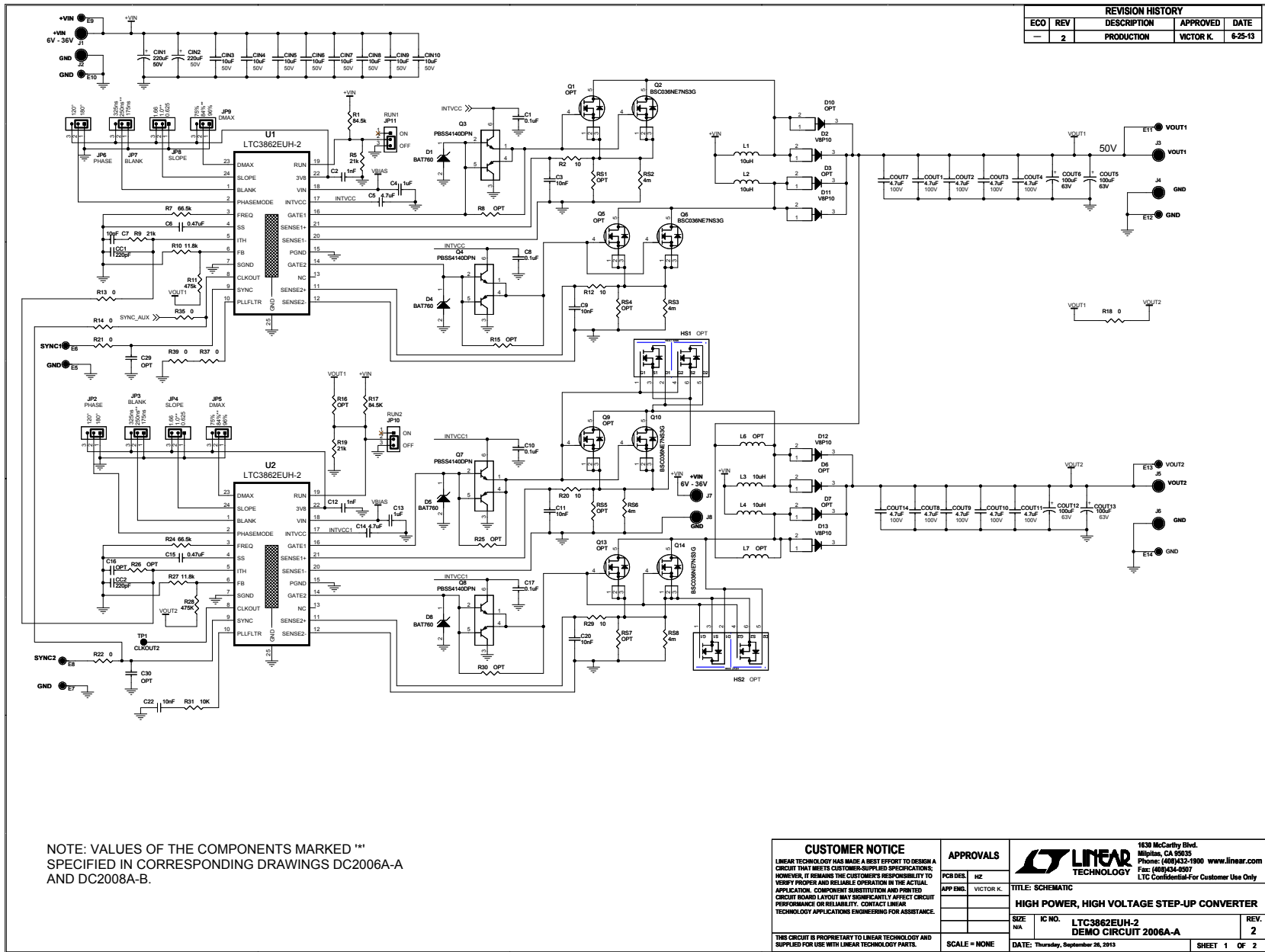
Figure 4. DC2006A-A Four-Phase Boost Converter
