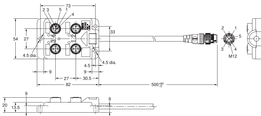
Connections Diagram
