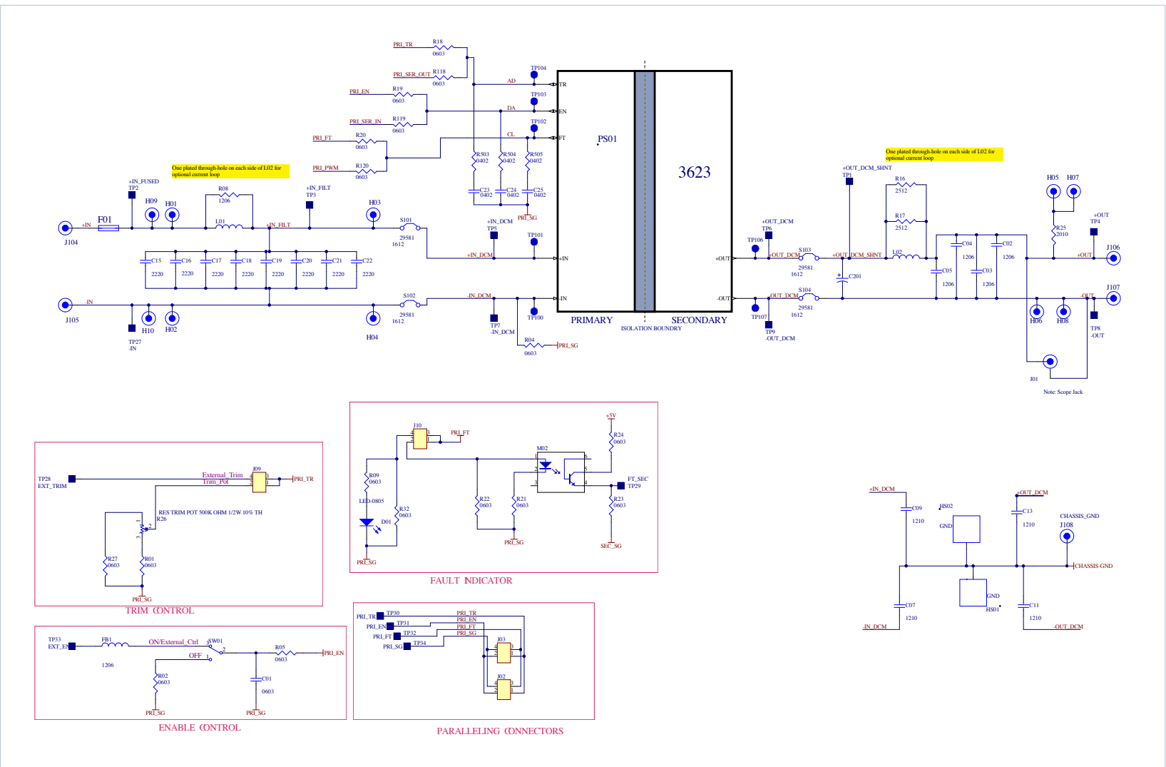
Figure 3 3623 DCM evaluation board schematic
