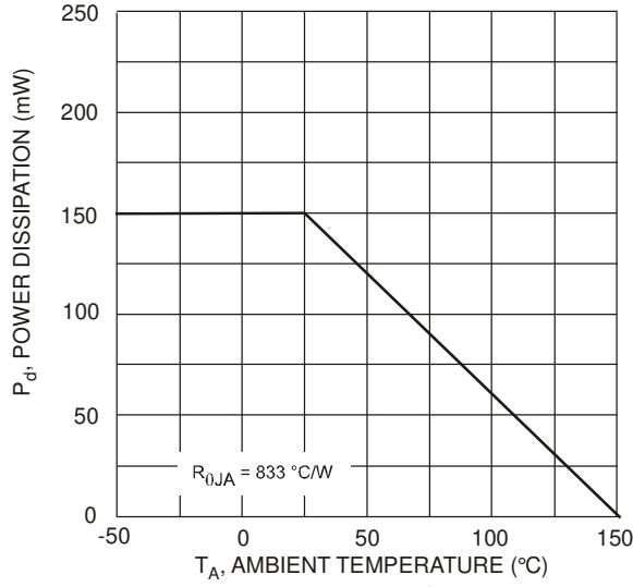
Fig. 1 Derating Curve
