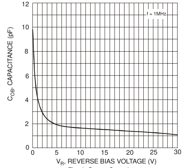
Fig. 4 Output Capacitance
