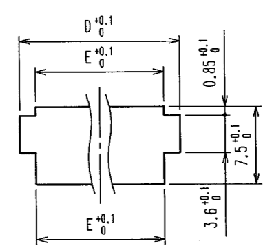
PANEL CUTOUT DIMENSIONS(2:1)
