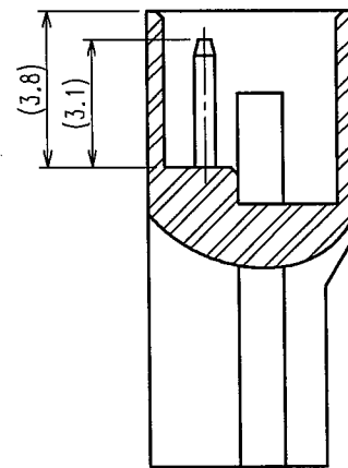
INSERTION FIGURE OF CRIMP CONTACT
