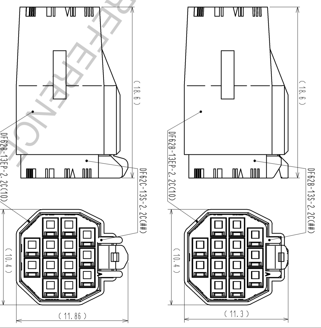
MATING FIGURE (FREE)
