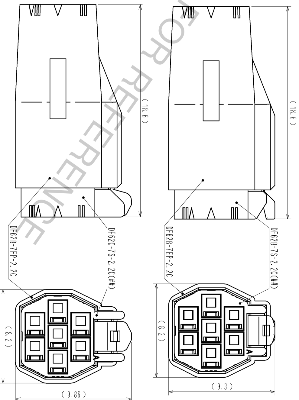
MATING FIGURE
