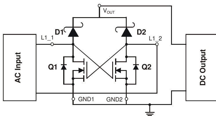
Figure 14 Typical Application Circuit GND1 and GND2 are not internally connected. The user should make the connection in the PCB design.
