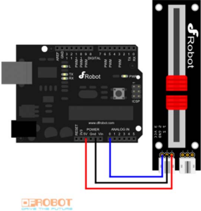
Analog sensor connection diagram
