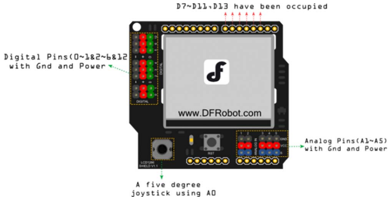
Instruction for Digital Pin 7 To 11,13 and Analog
