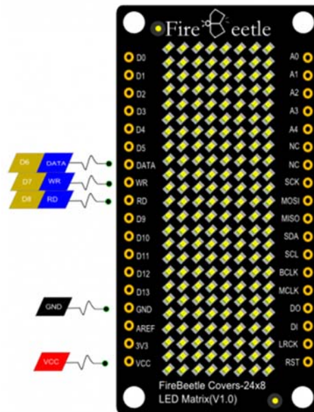
FireBeetle Covers-24x8 LED Matrix
