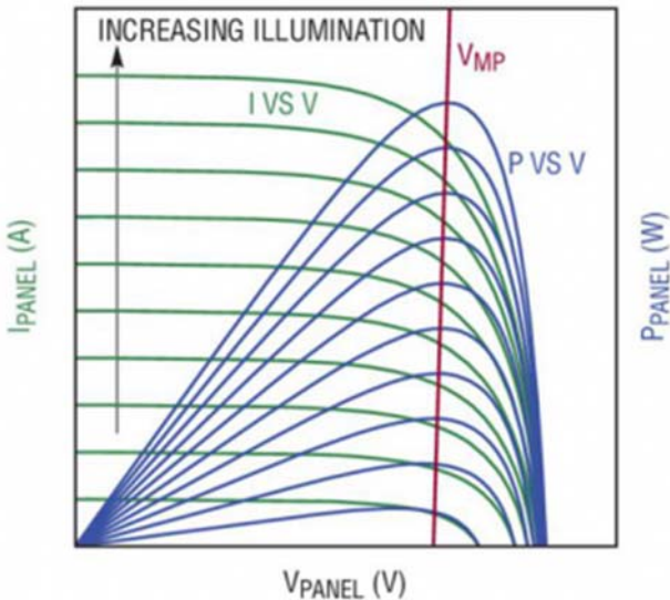
IV/PV characteristic curve of a typical solar panel (picture from Linear Technology)
