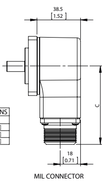
MIL CONNECTOR
