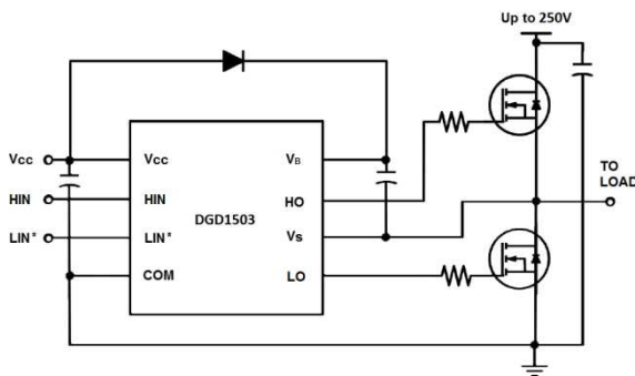
Typical Configuration
