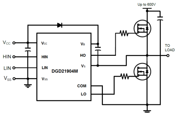
Typical Configuration
