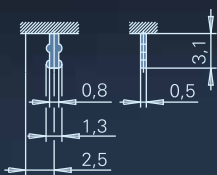
PCB terminal straight
