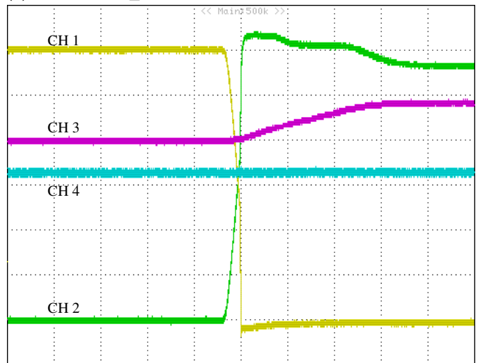
Figure 4: Oring for one feed loss (500μS/div): CH1: linA (1A/div) CH2: linB (1A/div). CH3: VRTN_OUT reference to -48V_OUT (10V/div). CH4: 3.3V (1V/div).
