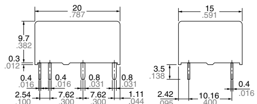
2 coil latching type
