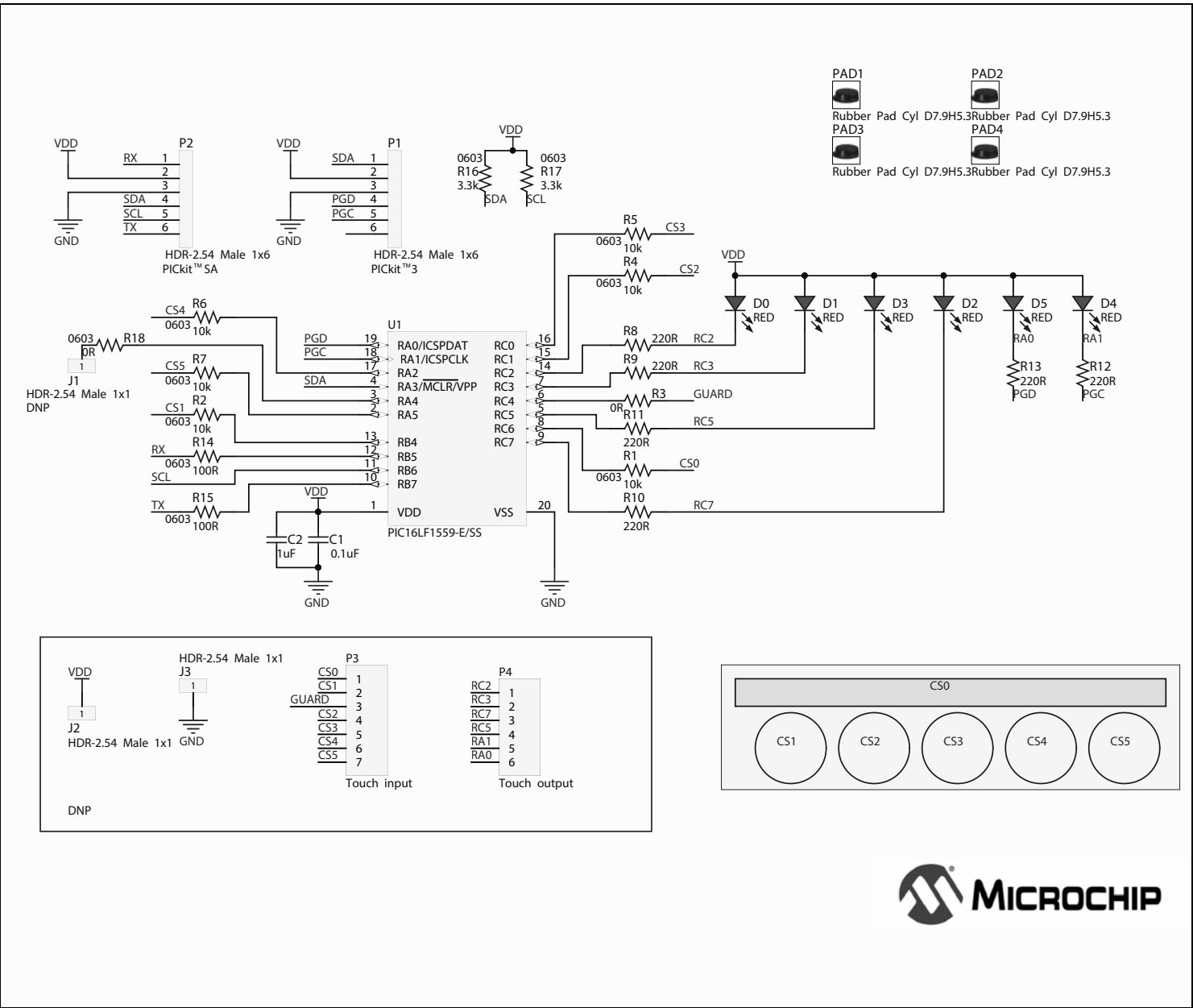
FIGURE A-1: LOW-COST mTouch® EVALUATION BOARD SCHEMATIC
