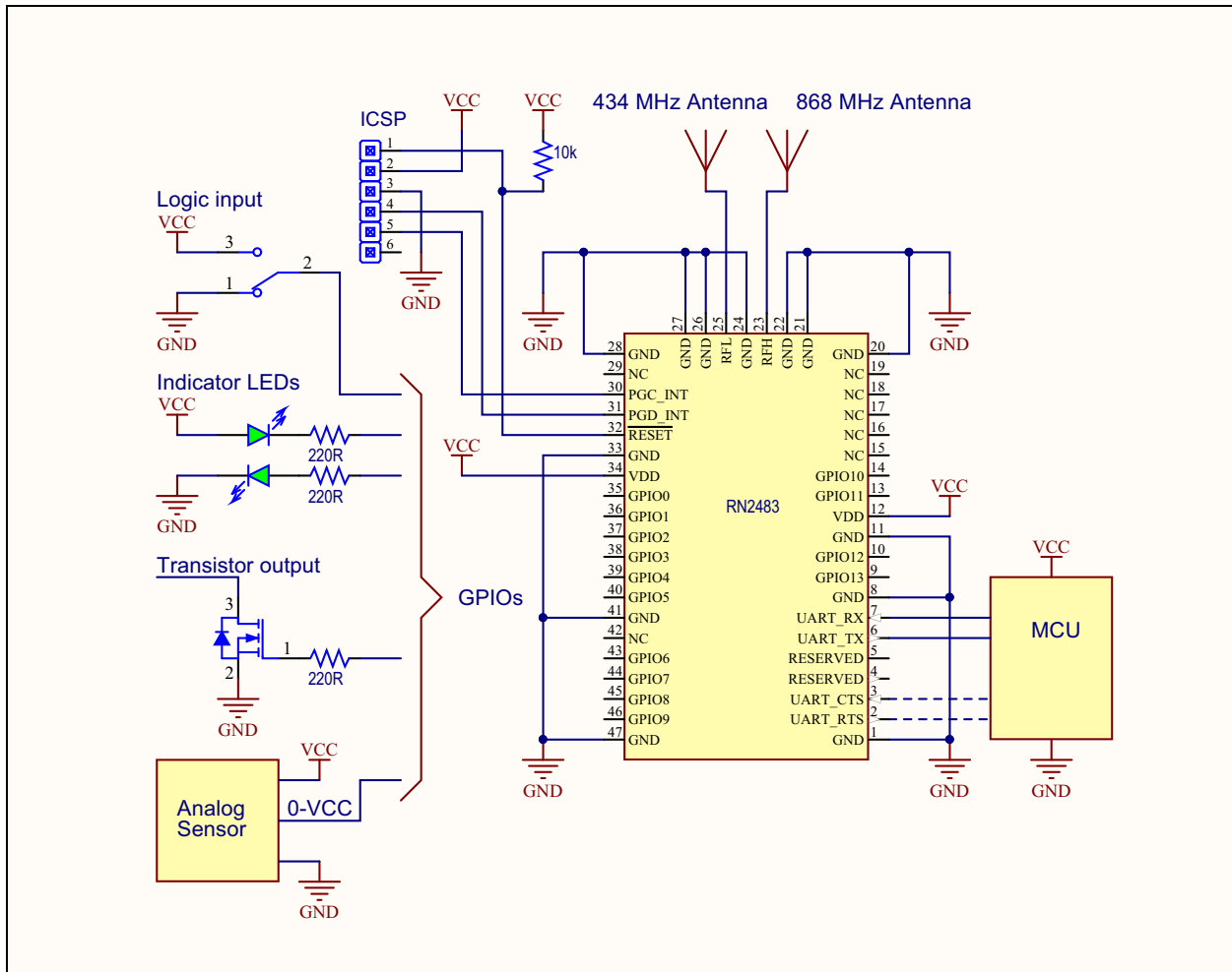
FIGURE 3-1: HARDWARE CONNECTIONS
