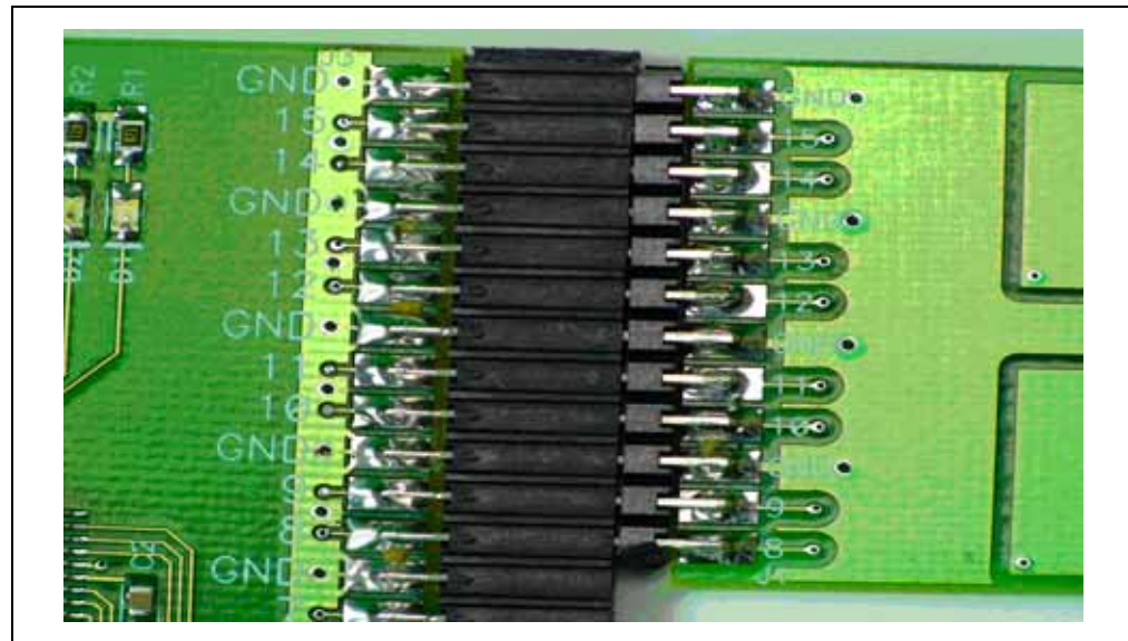
FIGURE 2-1: DEFAULT PLUG-IN CHANNELS FOR 8-KEY PLUG-IN BOARD
