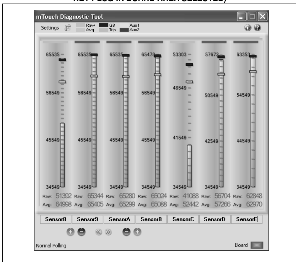
FIGURE 3-3: DIAGNOSTIC TOOL WINDOW FOR mTouch™ SENSING SOLUTION WITH SUCCESSFUL USB CONNECTION (MATRIX KEY PLUG-IN BOARD AREA SELECTED)
