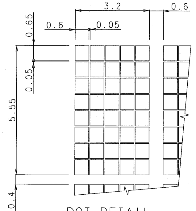
DOT DETAIL SCALE 10:1
