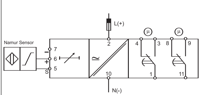
PMC01D - Namur sensor input
