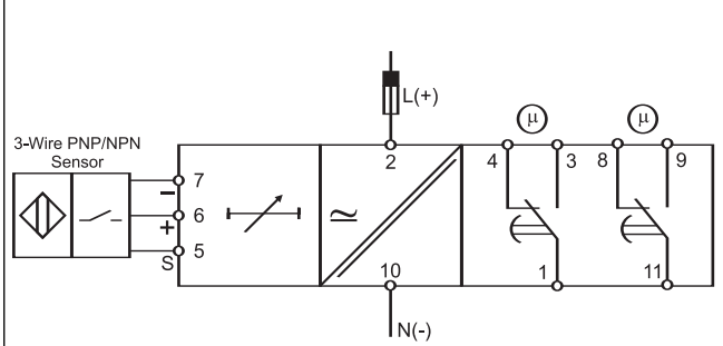
PMC01D - PNP / NPN sensor input
