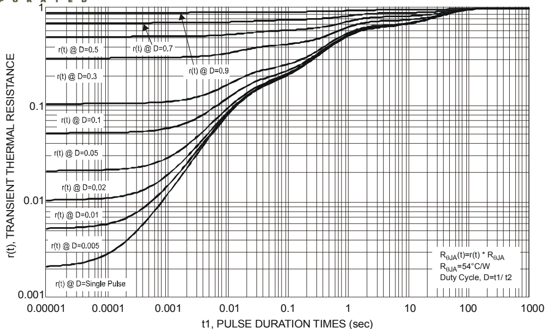
Fig. 12 Transient Thermal Resistance
