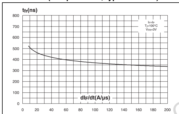
Figure 13. Forward recovery time vs. di_F/dt (damper diode, typical values)
