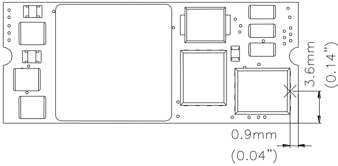
Figure 31: Temperature measurement location The allowed maximum hot spot temperature is defined at 125°C
