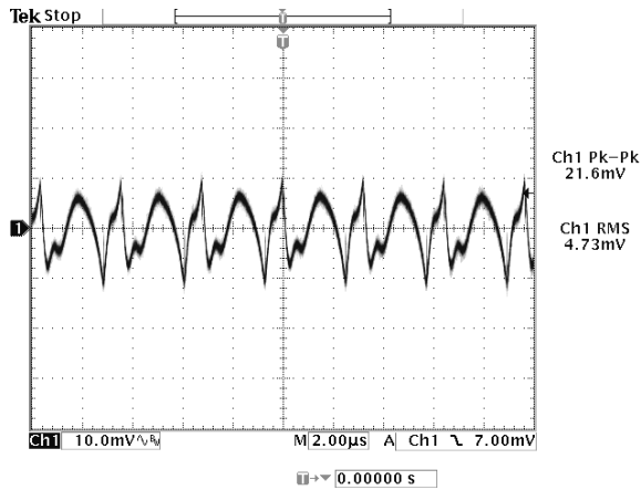
Figure 8: Output ripple & noise at 12Vin, 2.5V/10A out
