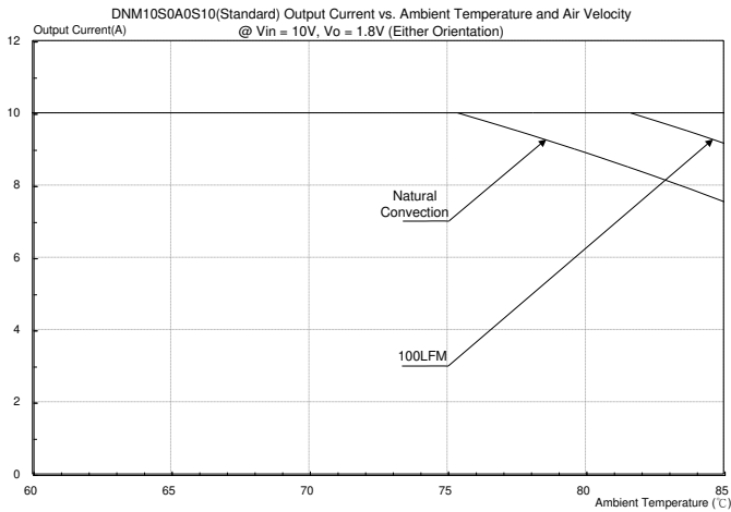
Figure 33: DNM10S0A0S10(Standard) Output current vs. ambient temperature and air velocity@ Vin=10V, Vo=1.8V(Either Orientation) DS_DNM10SMD10_07182012
