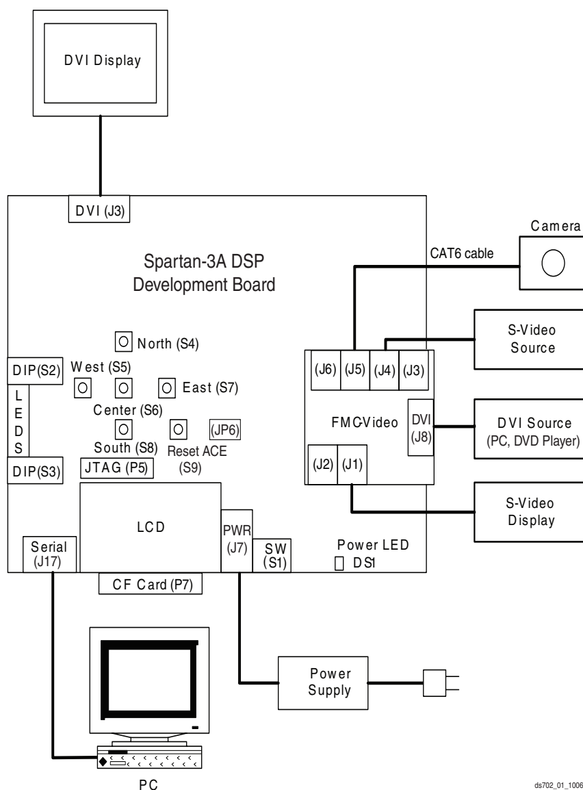
Figure 1-1: Video Starter Kit Physical Setup
