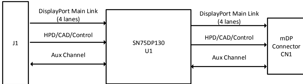
Figure 2.1 Functional Block Diagram
