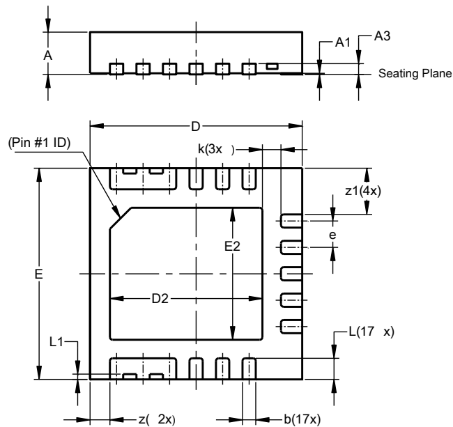
V-QFN4040-17
