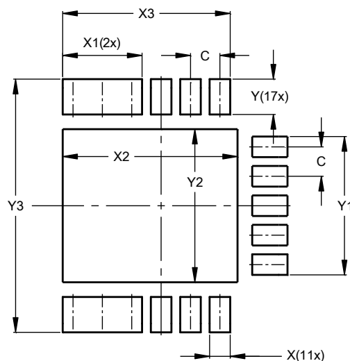
V-QFN4040-17
