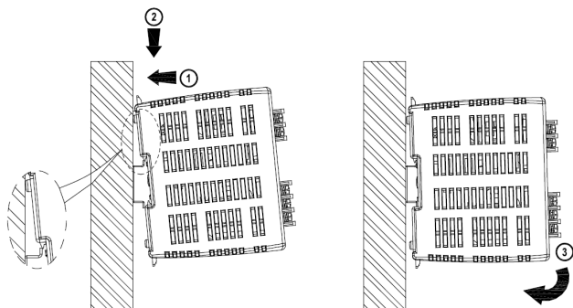
Fig. 2.1 Mounting
