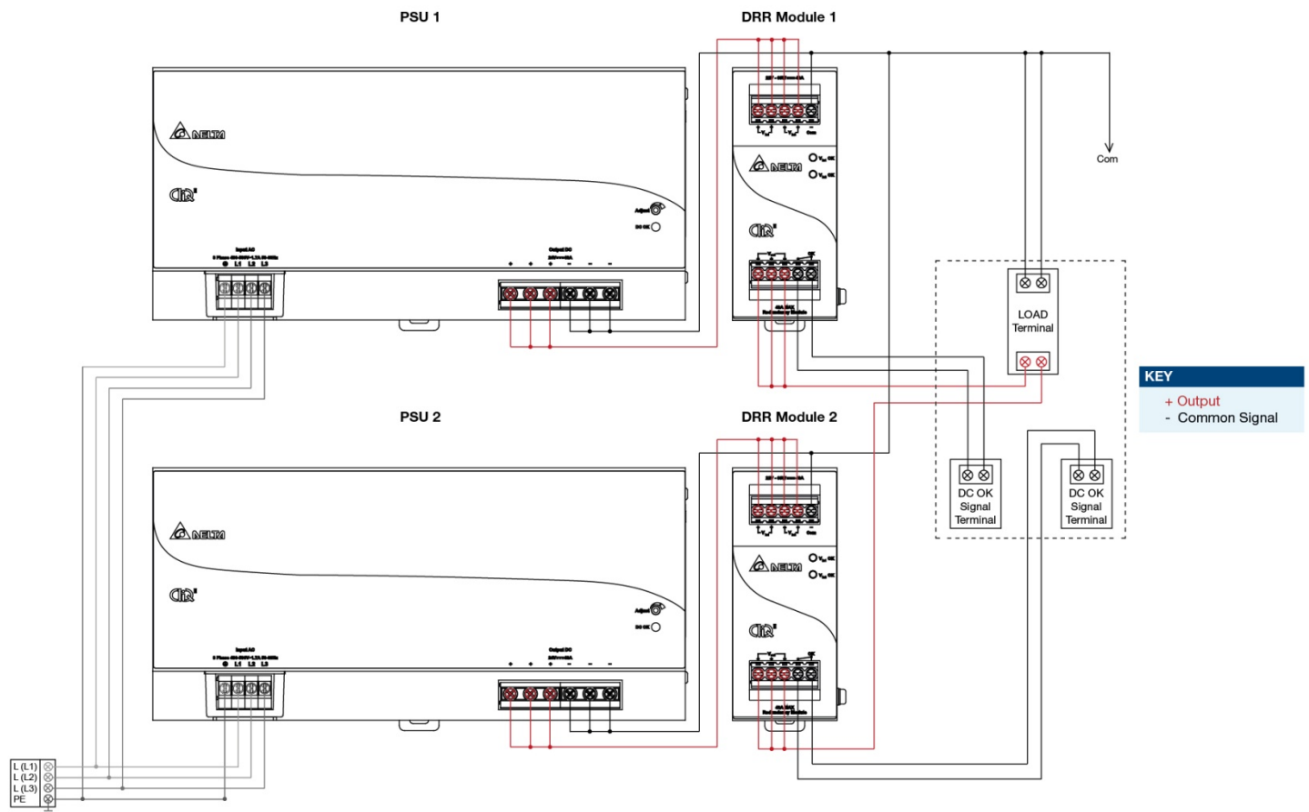
Fig. 3 Redundancy / Parallel Operation Connection Diagram
