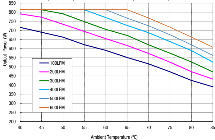
Dual Output Pins Maximum Output Power Temperature Derating at sea level (Vin = 48V, airflow from Vin to Vout, with heatsink)*
