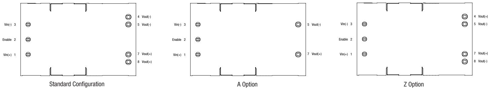
Figure 1. Bottom View of typical unit Pin-out Options
