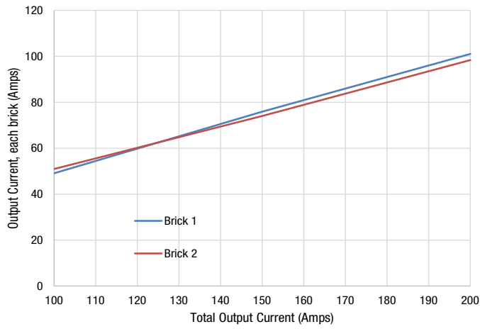
Current Share@ +25°C
