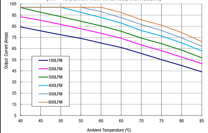
Single Output Pins Maximum Current Temperature Derating at sea level (Vin = 48V, airflow from Vin to Vout, with heatsink)*
