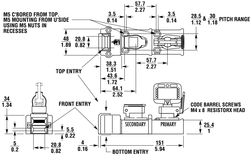
Standard Actuator
