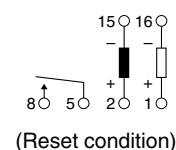
Schematic (Bottom view) Single side stable 2 coil latching
