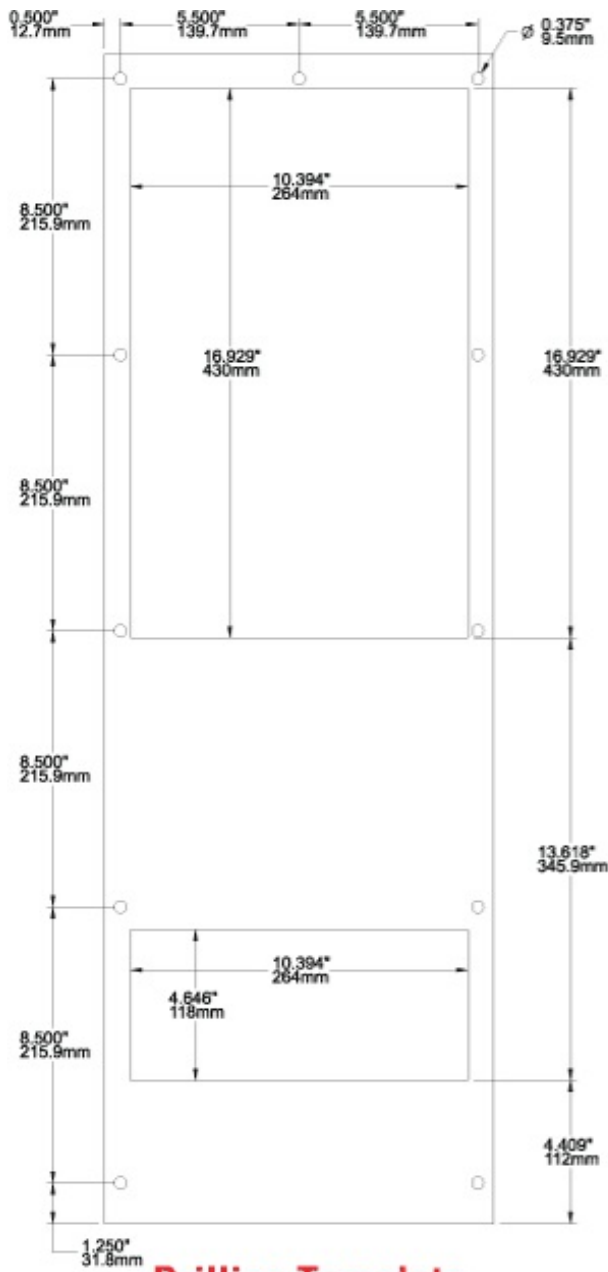
Drilling Template
