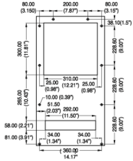
Drilling Template
