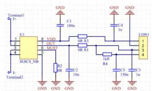
PCB schematic
