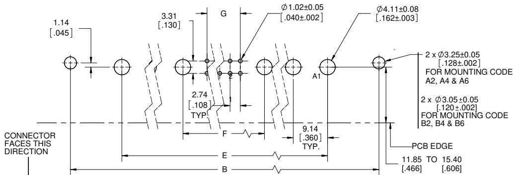
RECOMMENDED PCB LAYOUT COMPONENT SIDE OF BOARD
