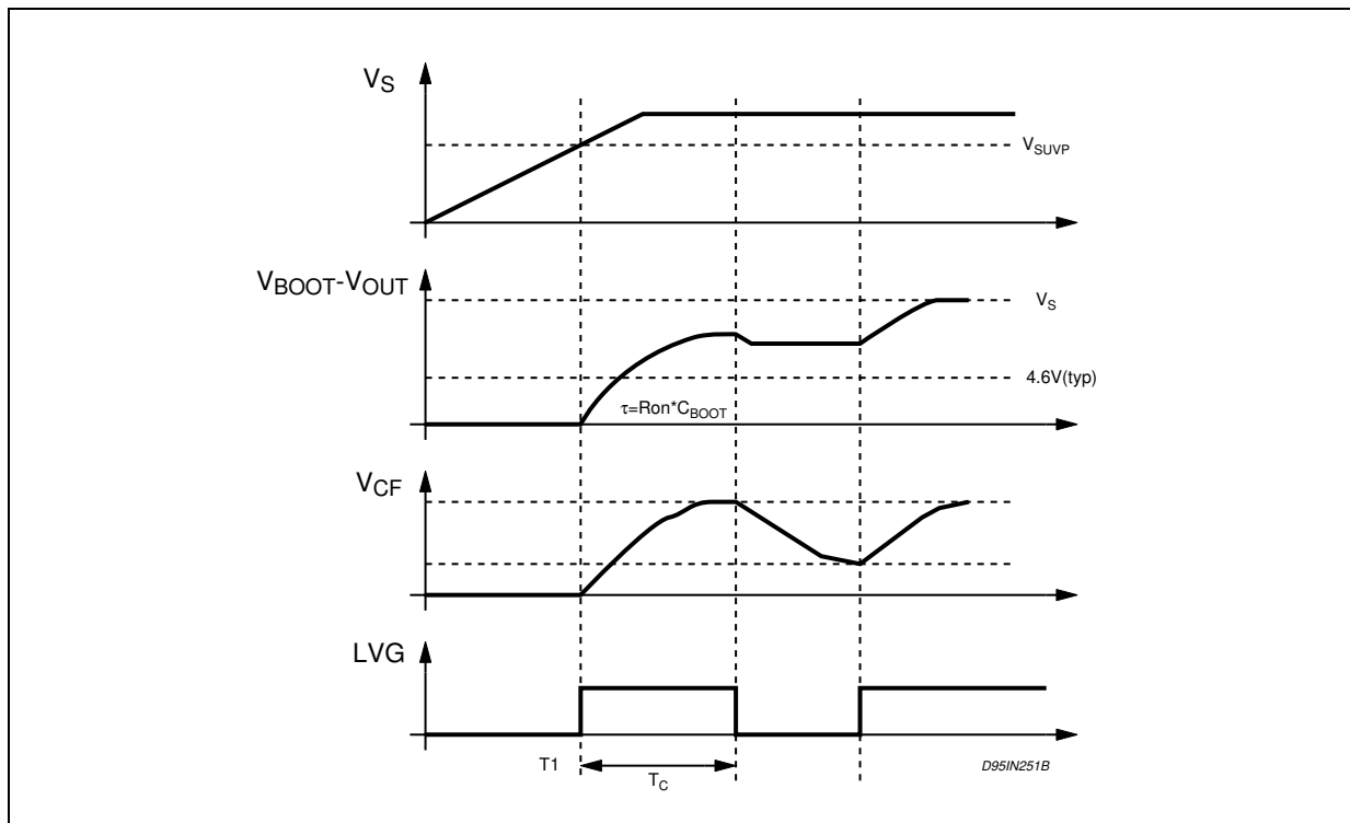
Figure 3. Waveforms (L6569A)
