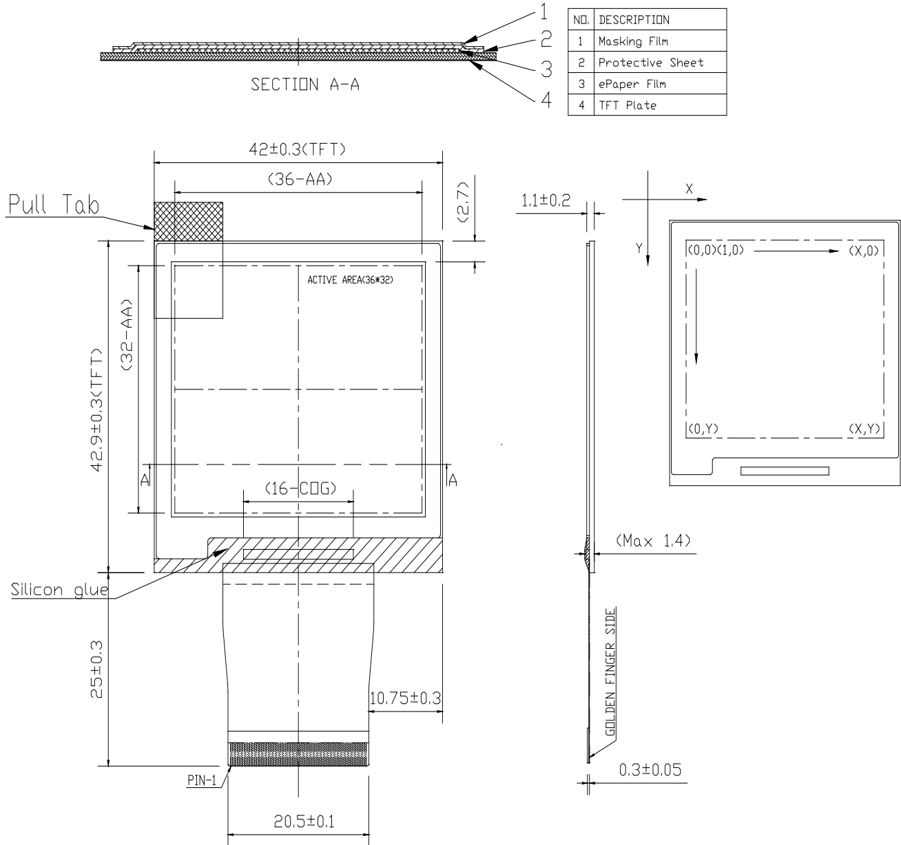
Figure 1-1 EPD Drawing
