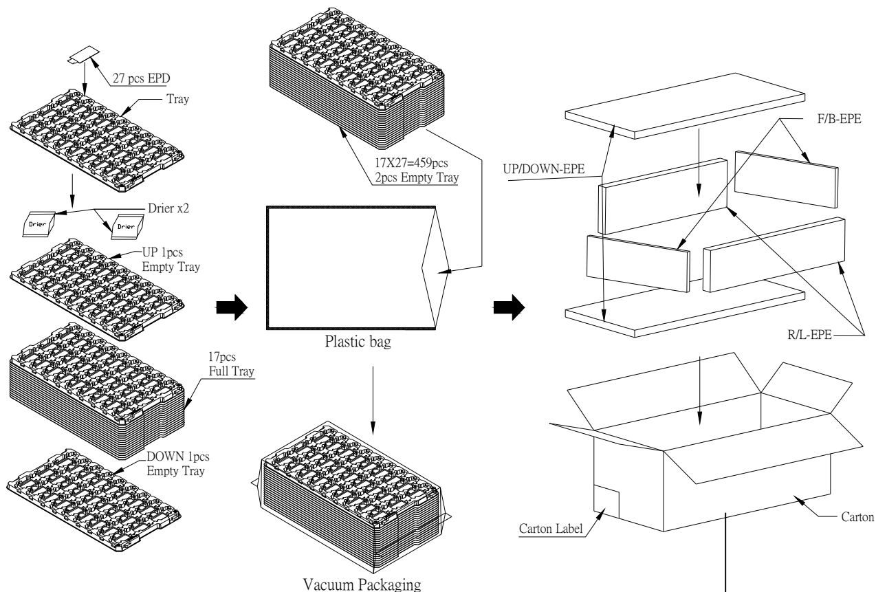
Figure 7-1 Packing Diagram
