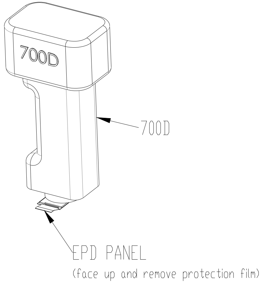
Figure 6-1 Optical measurement
