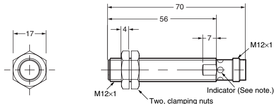
E2AU-M12LS04-M1-□□
