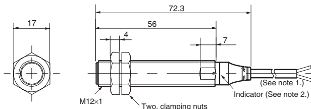
E2A-M12LS04-WP-□□
