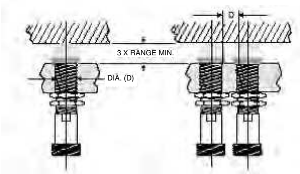
MINIMUM SPACING REQUIRED D (DIAMETER OF SENSOR)
