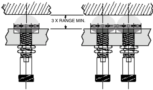
MINIMUM SPACING REQUIRED 2xD (DIAMETER OF SENSOR)
