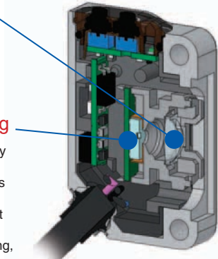
Cross Section
