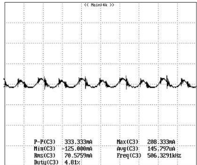
Figure 12: Input Terminal Ripple Current, i_o , at full rated output current and nominal input voltage with 12\mu H source impedance and 33\mu F electrolytic capacitor (500 mA/div, 2us/div).
