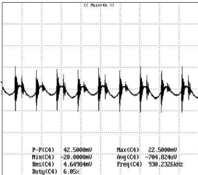
Figure 15: Output voltage ripple at nominal input voltage and rated load current ( I_o=10\text{A} ) ( 20\text{ mV/div} , 2\mu\text{s/div} ) Load capacitance: 1\mu\text{F} ceramic capacitor and 10\mu\text{F} tantalum capacitor. Bandwidth: 20\text{ MHz} . Scope measurements should be made using a BNC cable (length shorter than 20\text{ inches} ). Position the load between 51\text{ mm} to 76\text{ mm} ( 2\text{ inches} to 3\text{ inches} ) from the module.
