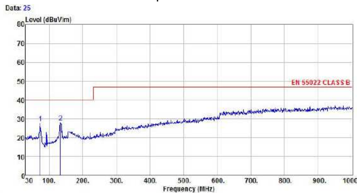
Vin=12V Output 9V2.4A Vertical
