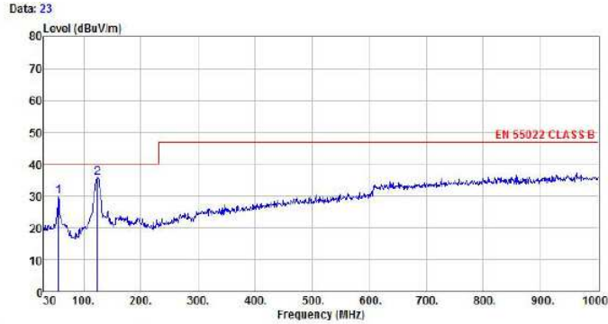
Vin=12V Output 5V2.4A Horizontal
