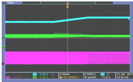
Vin=12V,Iout=0A,Vout 9V→12V
