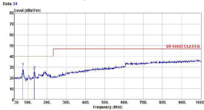
Vin=12V Output 9V2.4A Horizontal
