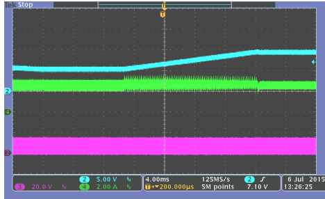
Vin=12V,Iout=2.4A,Vout 5V→9V
