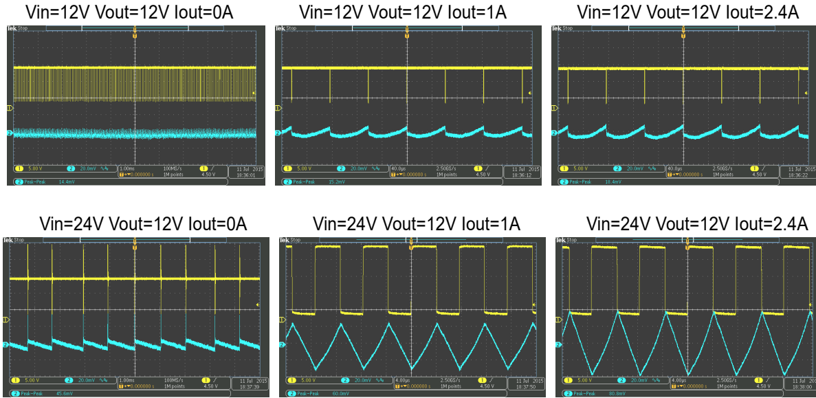
Ripple & noise are measured by using 20MHz bandwidth limited oscilloscope
