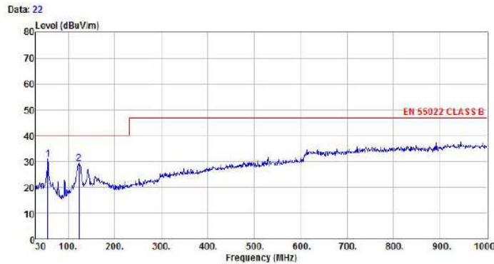
Vin=12V Output 5V2.4A Vertical
