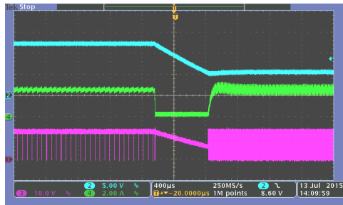
Vin=12V,Iout=0A,Vout 12V→5V
