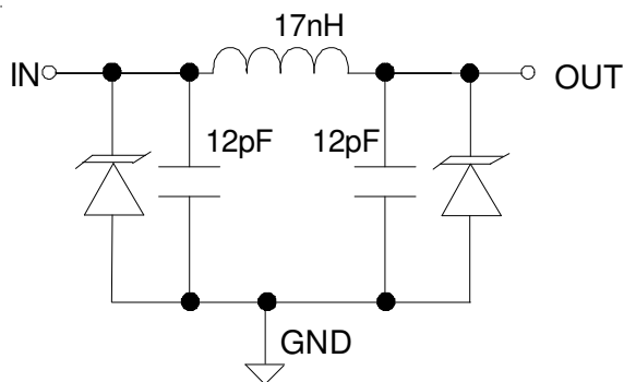
Device Schematic (8X)
